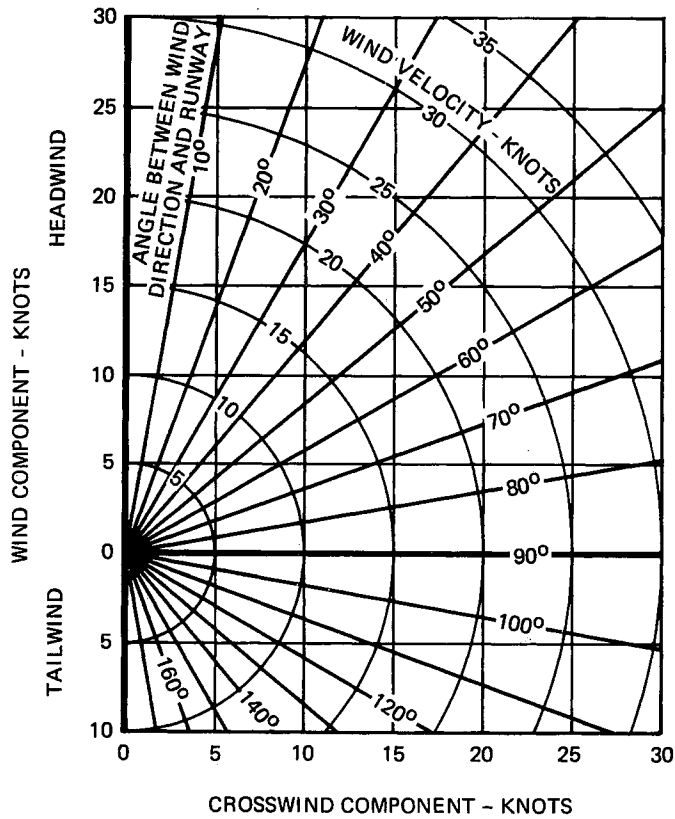
Figure 5-4. Wind Components
