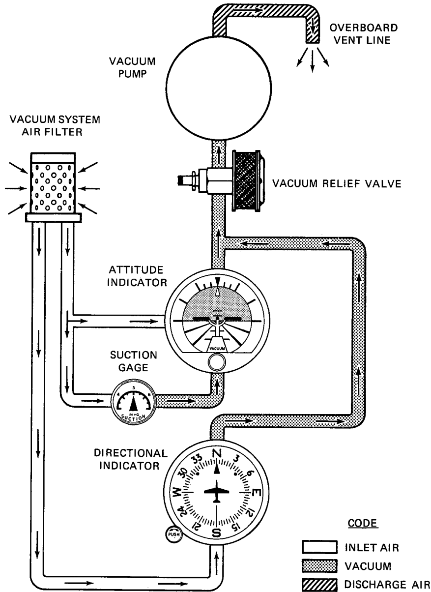
Figure 7-9. Vacuum System
